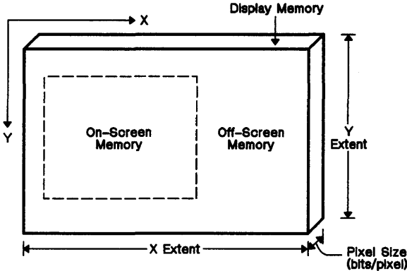
Figure 4-7. Display Memory Dimensions
