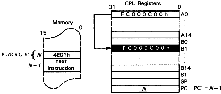
Figure 12-3. An Example of Register-Direct Addressing
