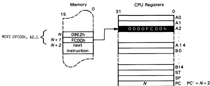
Figure 12-1. An Example of Immediate Addressing
