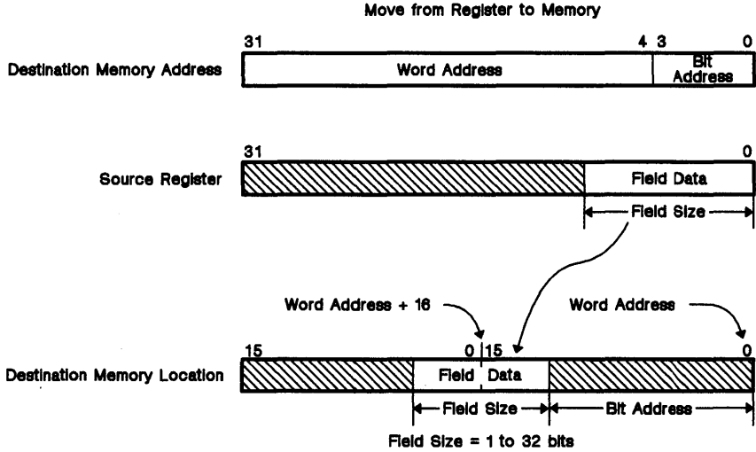
Figure 12-8. Register-to-Memory Moves
