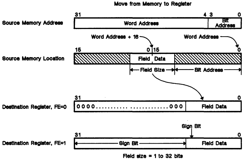
Figure 12-9. Memory-to-Register Moves
