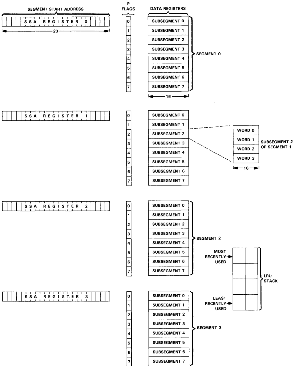
FIGURE 3. INSTRUCTION CACHE
