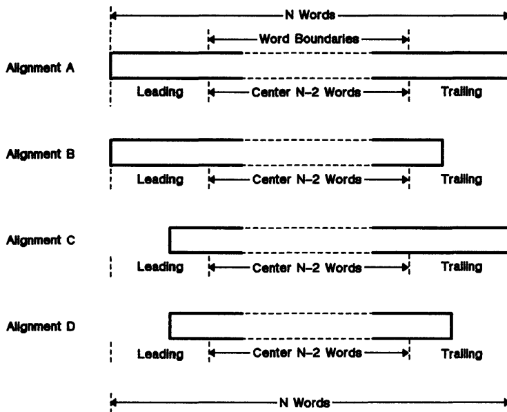
Figure 13-9. Pixel Block Alignments
