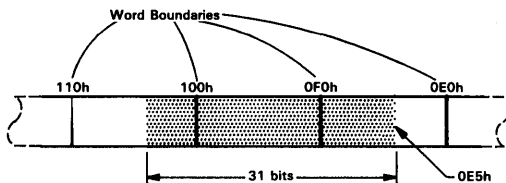
Figure 13-2. Source Data, Alignment G
