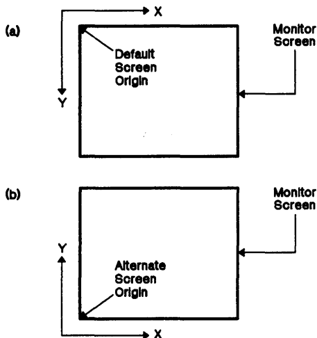
Figure 4-6. Configurable Screen Origin
