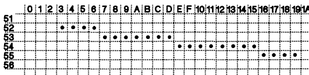
Figure 12-12. LINE Timing Example
